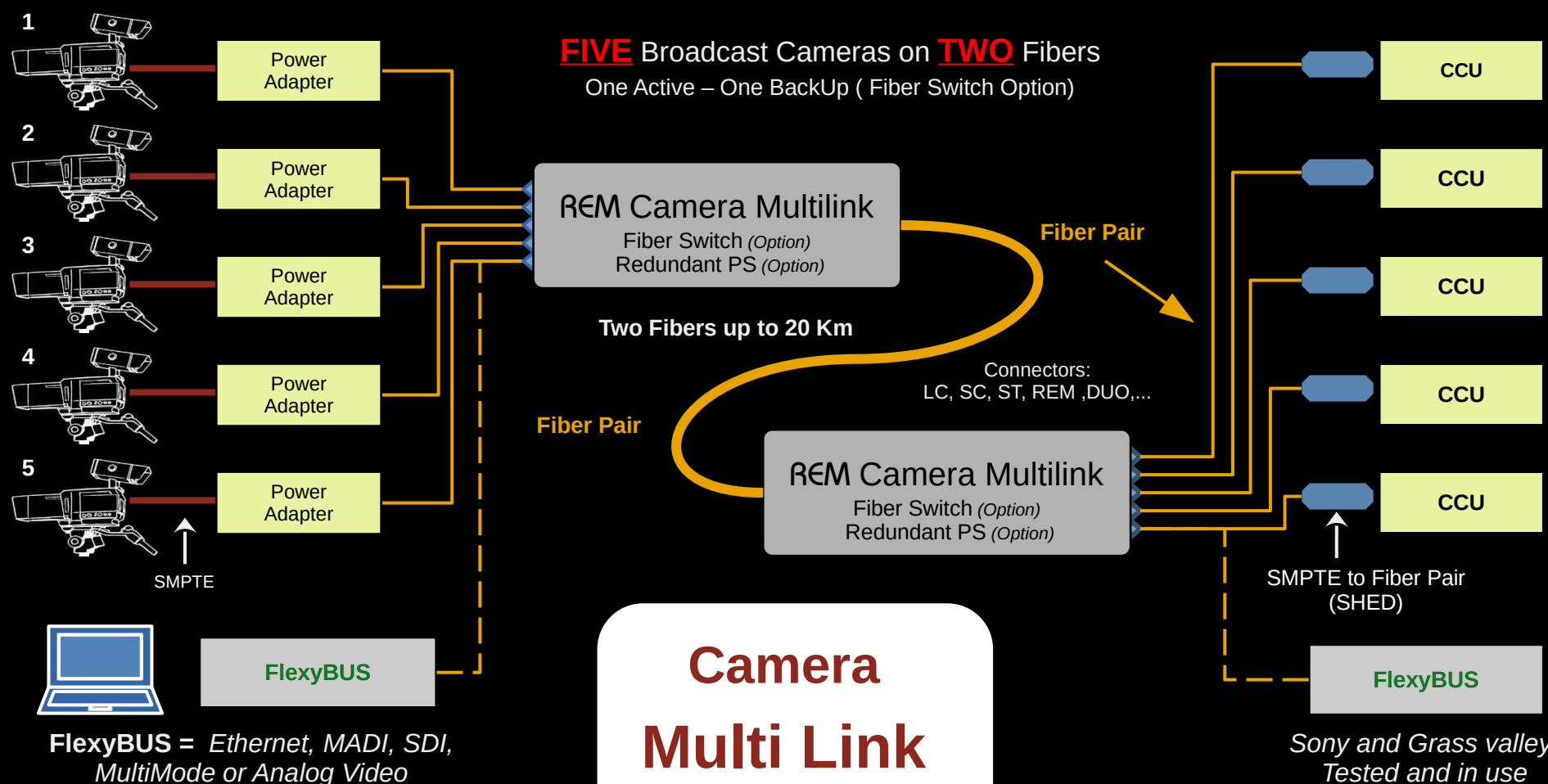
Fiber Switch
